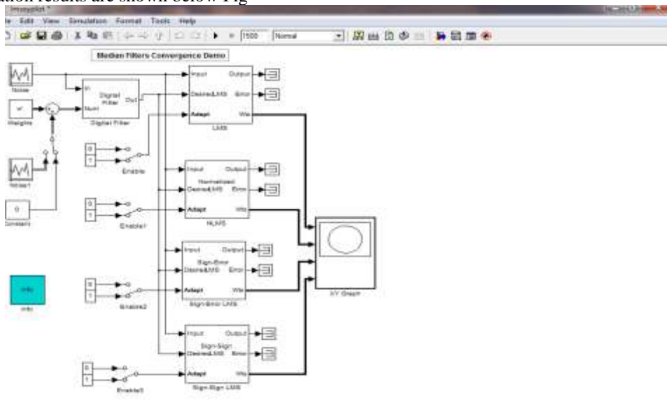
Fig 3. Simulink Simulation
