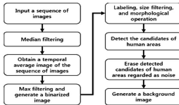
Fig 2. Flow Chart
